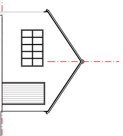
SURVEY - EAST ELEVATION scale 1/100 @ A3
