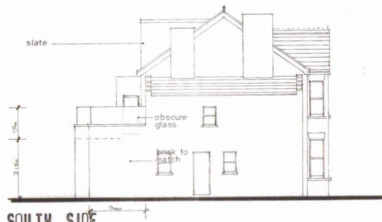
SOUTH SIDE
