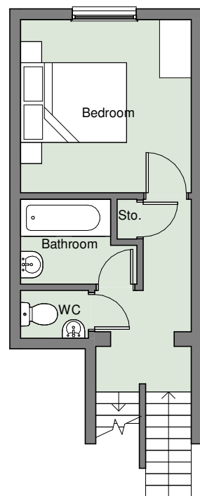
2 Proposed First Floor Plan 1 : 100
