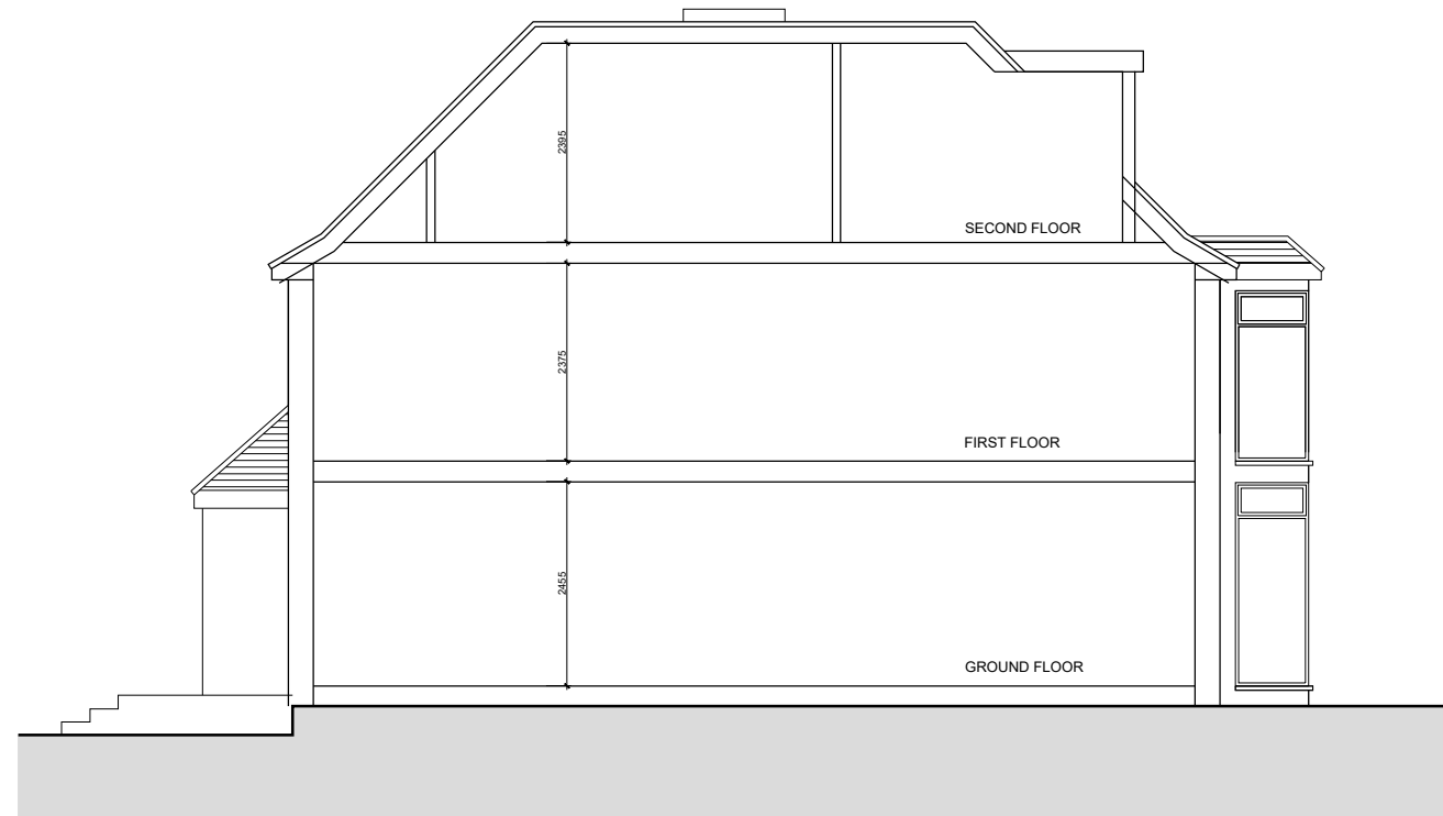
1 EXISTING TYPICAL SECTION SK-023 SCALE@A1 1:50 SCALE@A3 1:100
