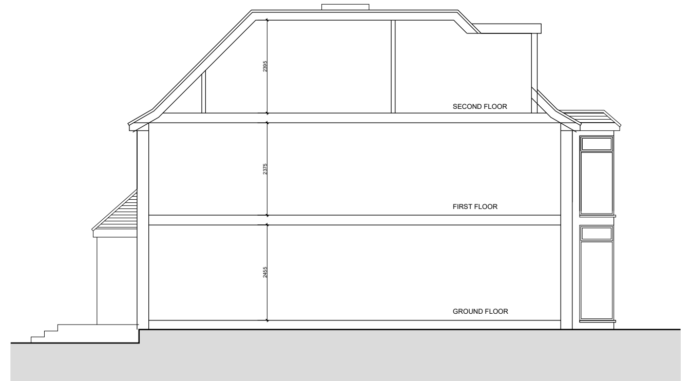
2 PROPOSED TYPICAL SECTION SK-023 SCALE@A1 1:50 SCALE@A3 1:100
