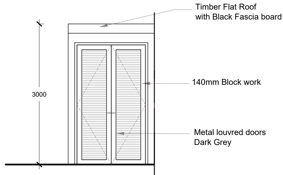
External Cycle Enclosure - Elevations 1:50
