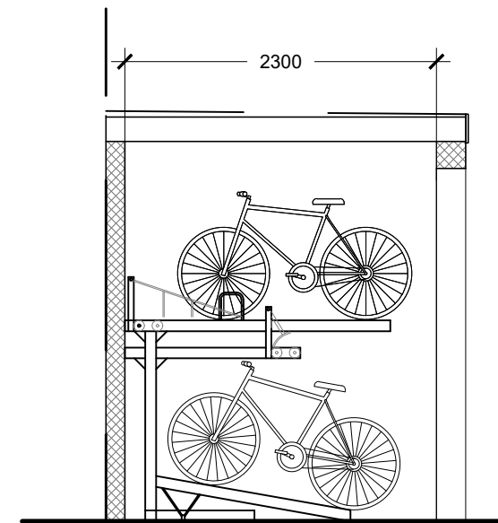
External Cycle Enclosure - Section AA 'JOSTA' Double Rack 1:50
