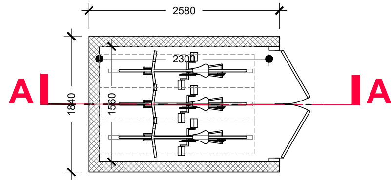
External Cycle Enclosure - Plan 1:50
