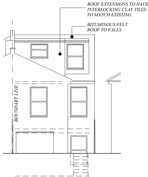
PROPOSED WEST ELEVATION
