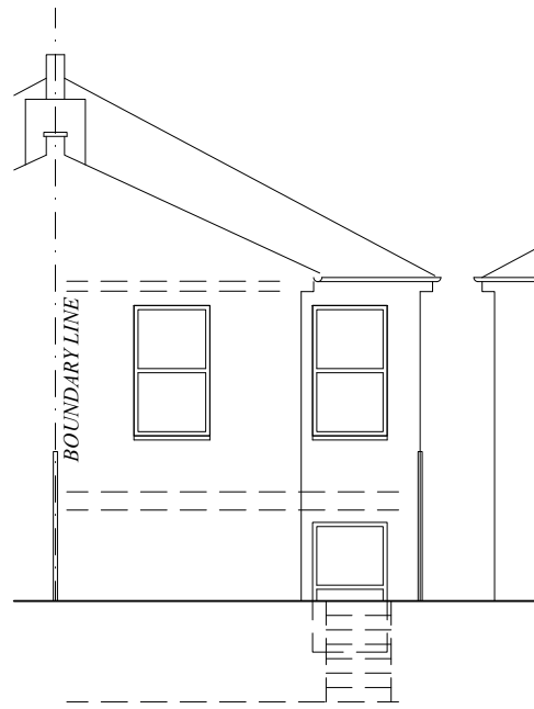
EXISTING WEST ELEVATION
