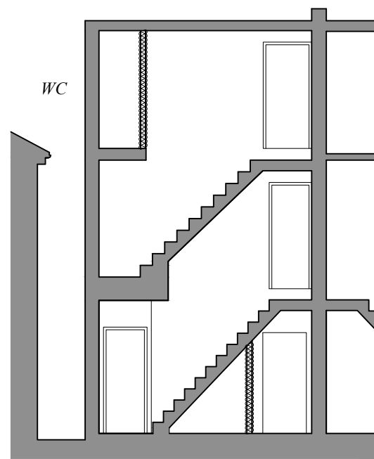
PROPOSED SECTION B-B
