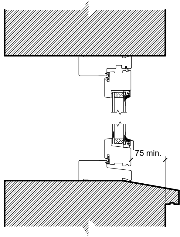
Typical Head/ Sill Detail
