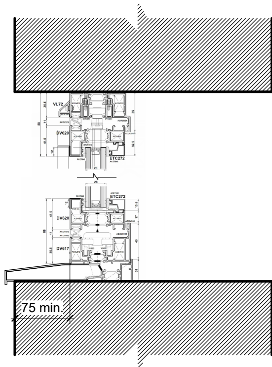
Typical Head/ Sill Detail
