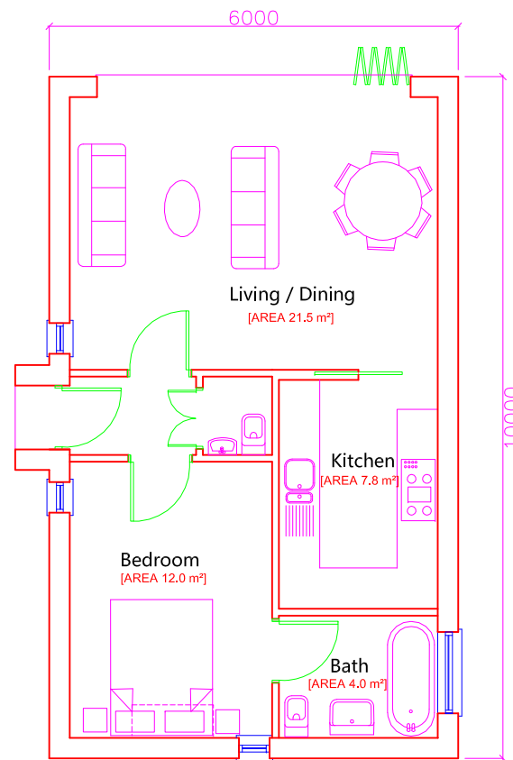
PROPOSED PLAN
