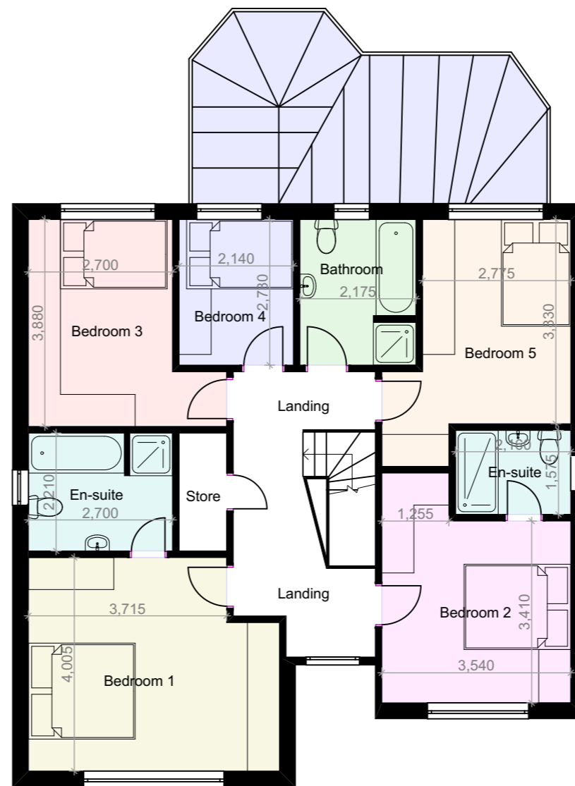
EXISTING GA FIRST FLOOR PLAN @ 1:100
