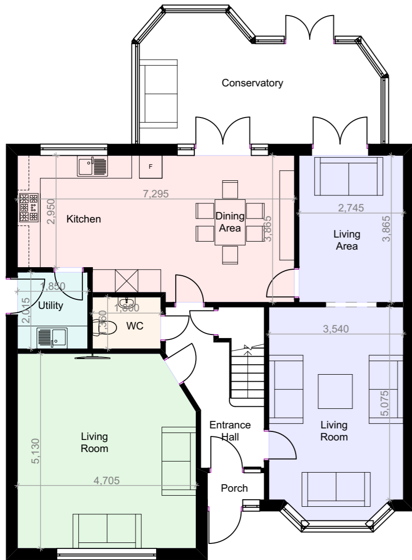
PROPOSED GA GROUND FLOOR PLAN @ 1:100
