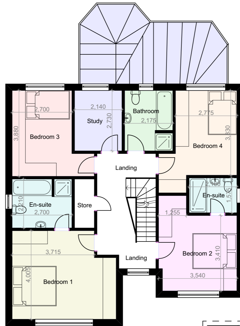
PROPOSED GA FIRST FLOOR PLAN @ 1:100
