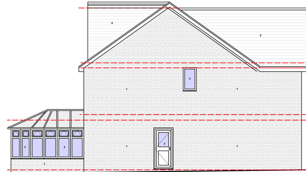
PROPOSED GA SIDE ELEVATION 2 @ 1:100
