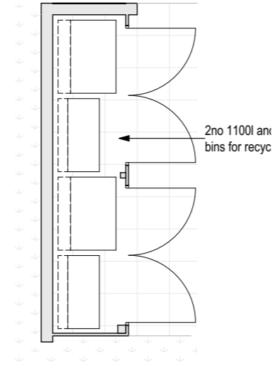
Bin Store 1:100
