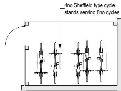
Cycle Store 1:100
