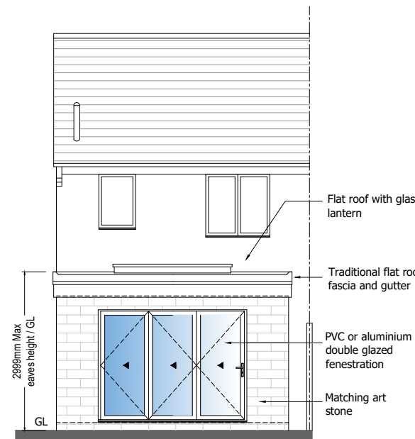
REAR ELEVATION (East facing)
