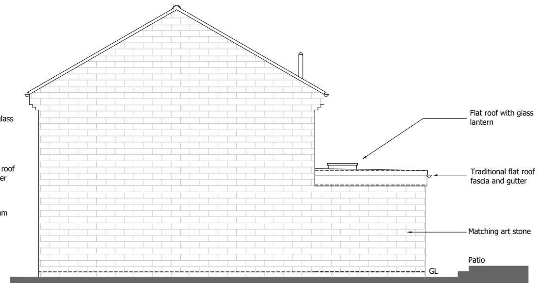
SIDE ELEVATION (South facing)
