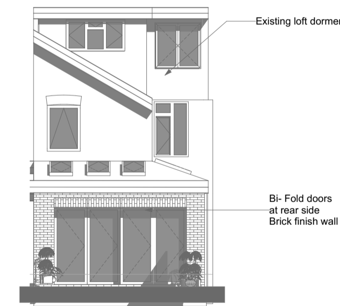
North Elevation @1:100
