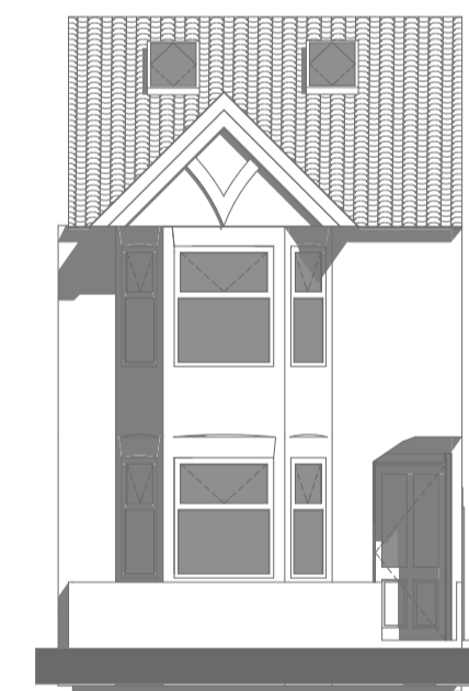
South Elevation @1:100
