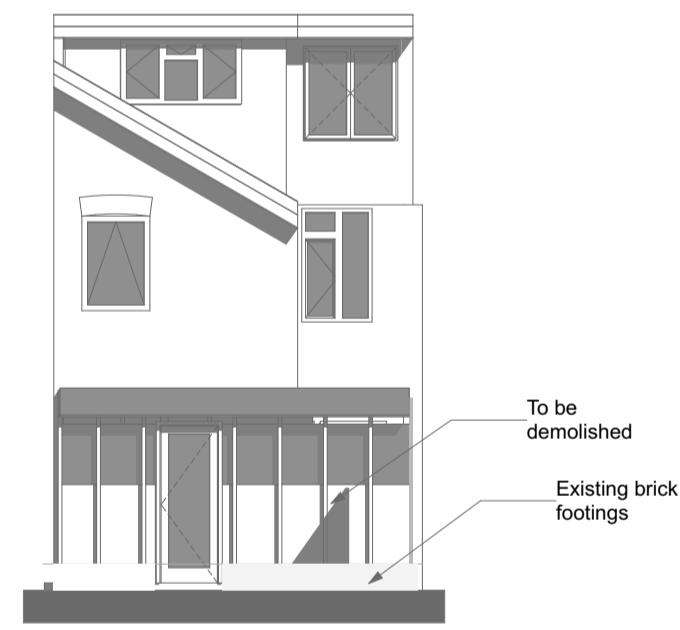
North Elevation @1:100
