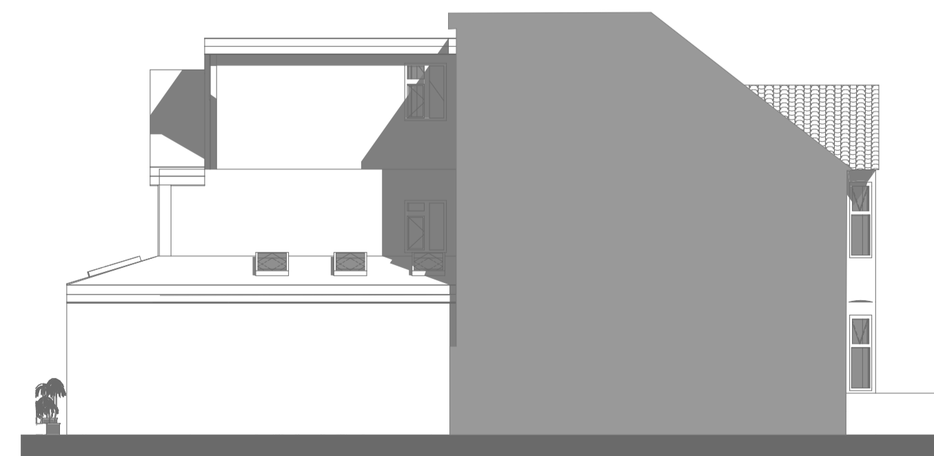
West Elevation @1:100
