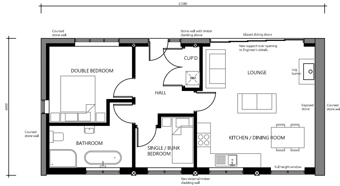
PROPOSED PLAN
