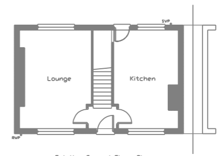
Existing Ground Floor Plan
