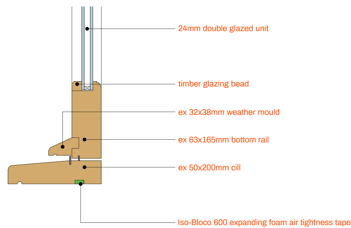
SECTION THROUGH DOOR CILL
