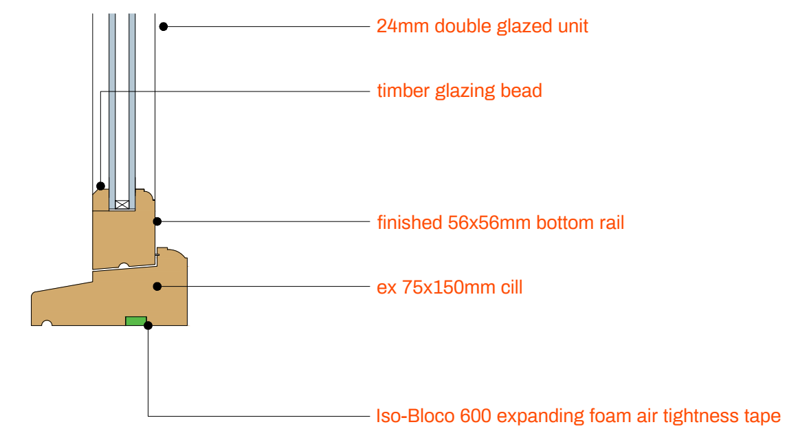
SECTION THROUGH WINDOW CILL
