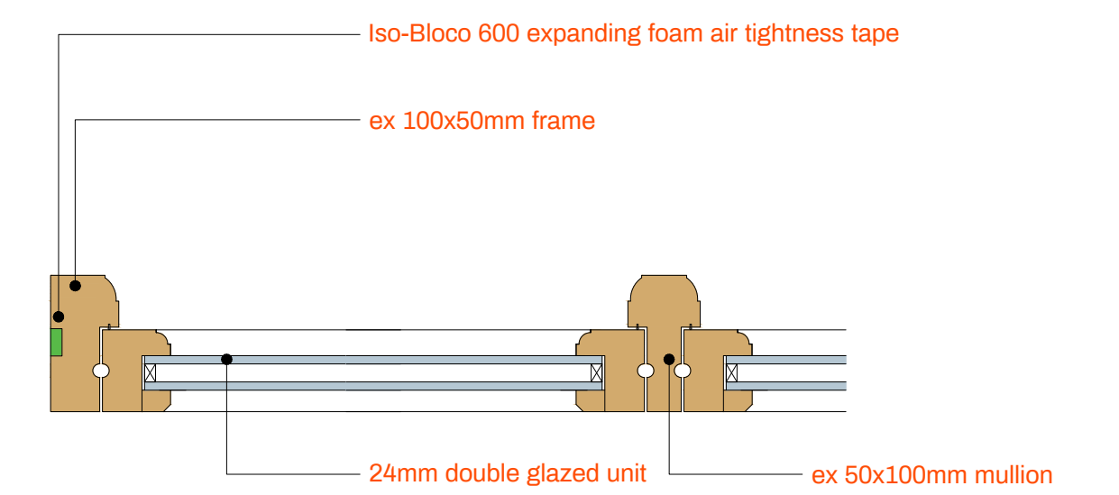
PLAN DETAIL THROUGH WINDOW JAMB
