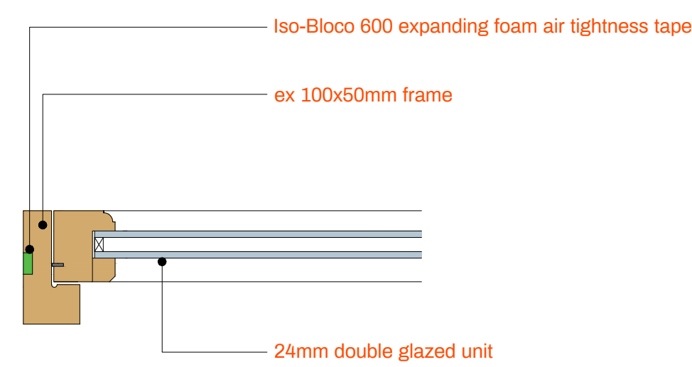
PLAN DETAIL THROUGH DOOR JAMB
