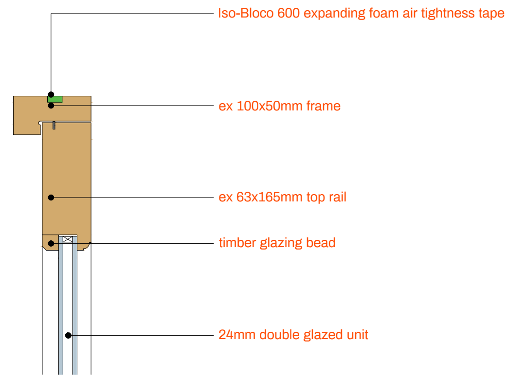
SECTION THROUGH DOOR HEAD
