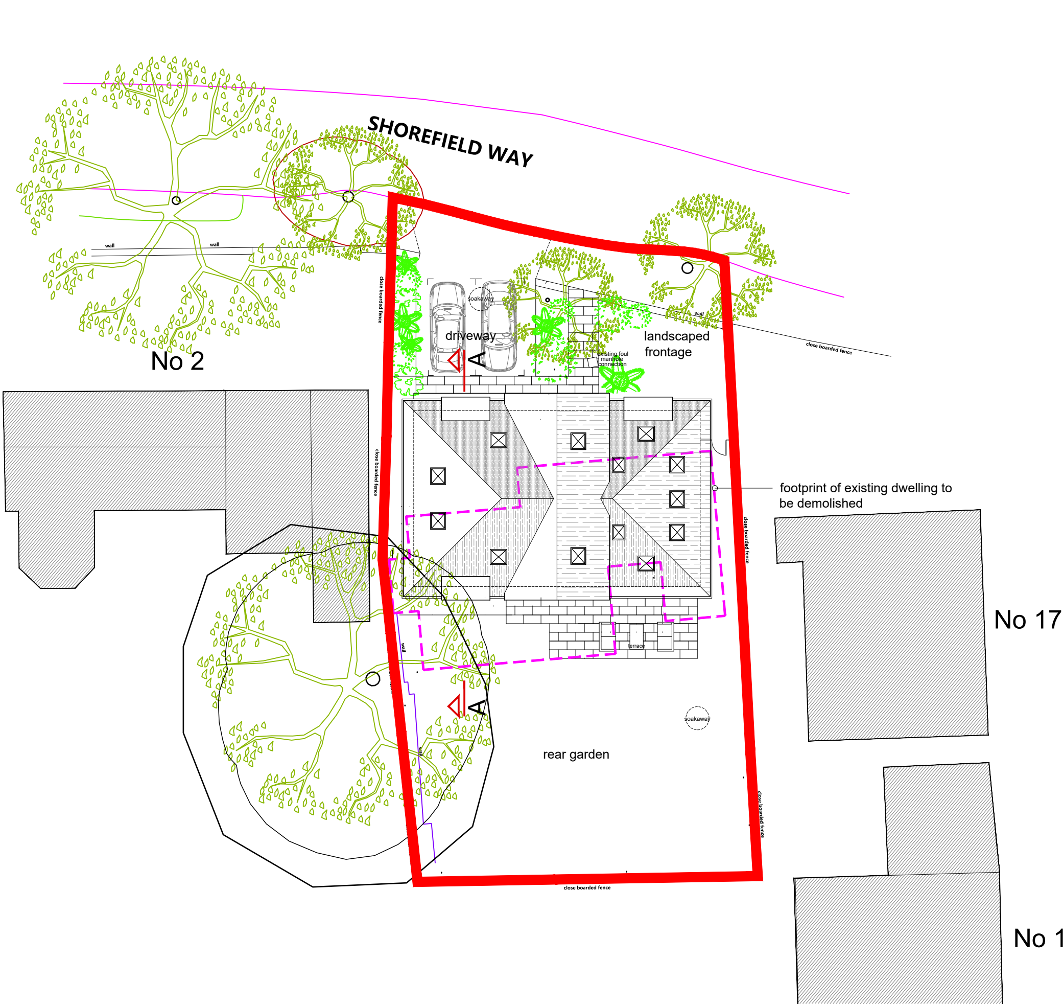
Proposed roofplan relative to oak tree existing v proposed dwelling relative to oak tree
