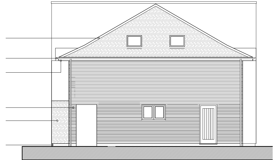
west elevation
