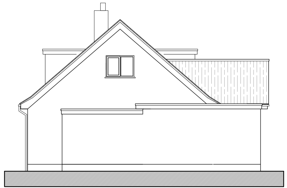
east elevation
