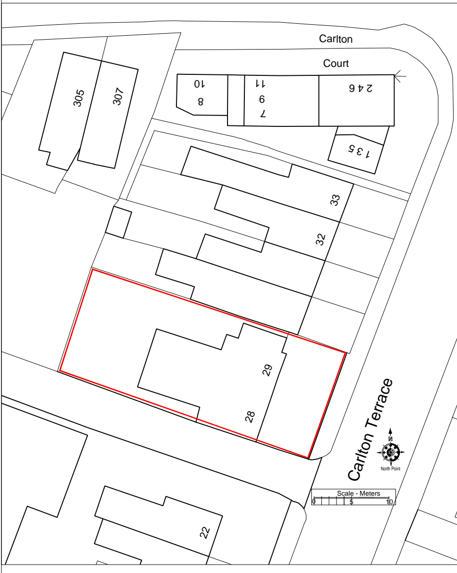
Block Plan 1:500
