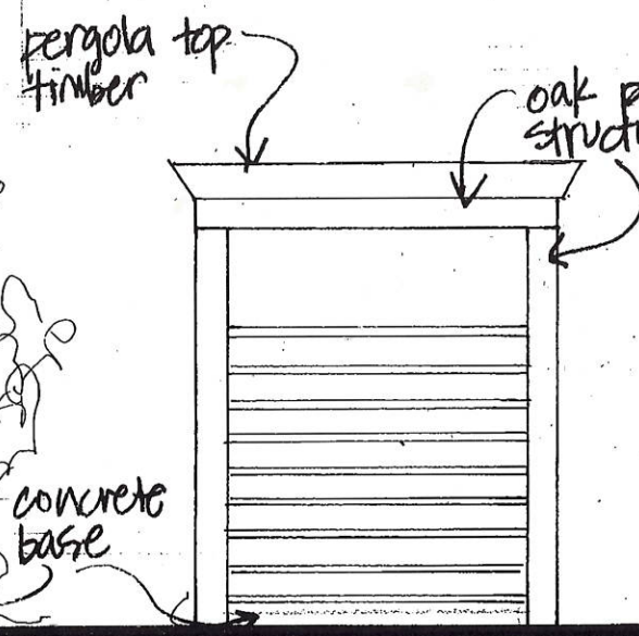
REAR ELEV 1:50
