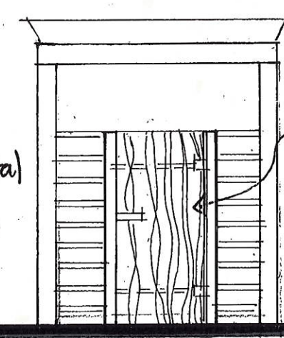
FRONT ELEV 1:50
