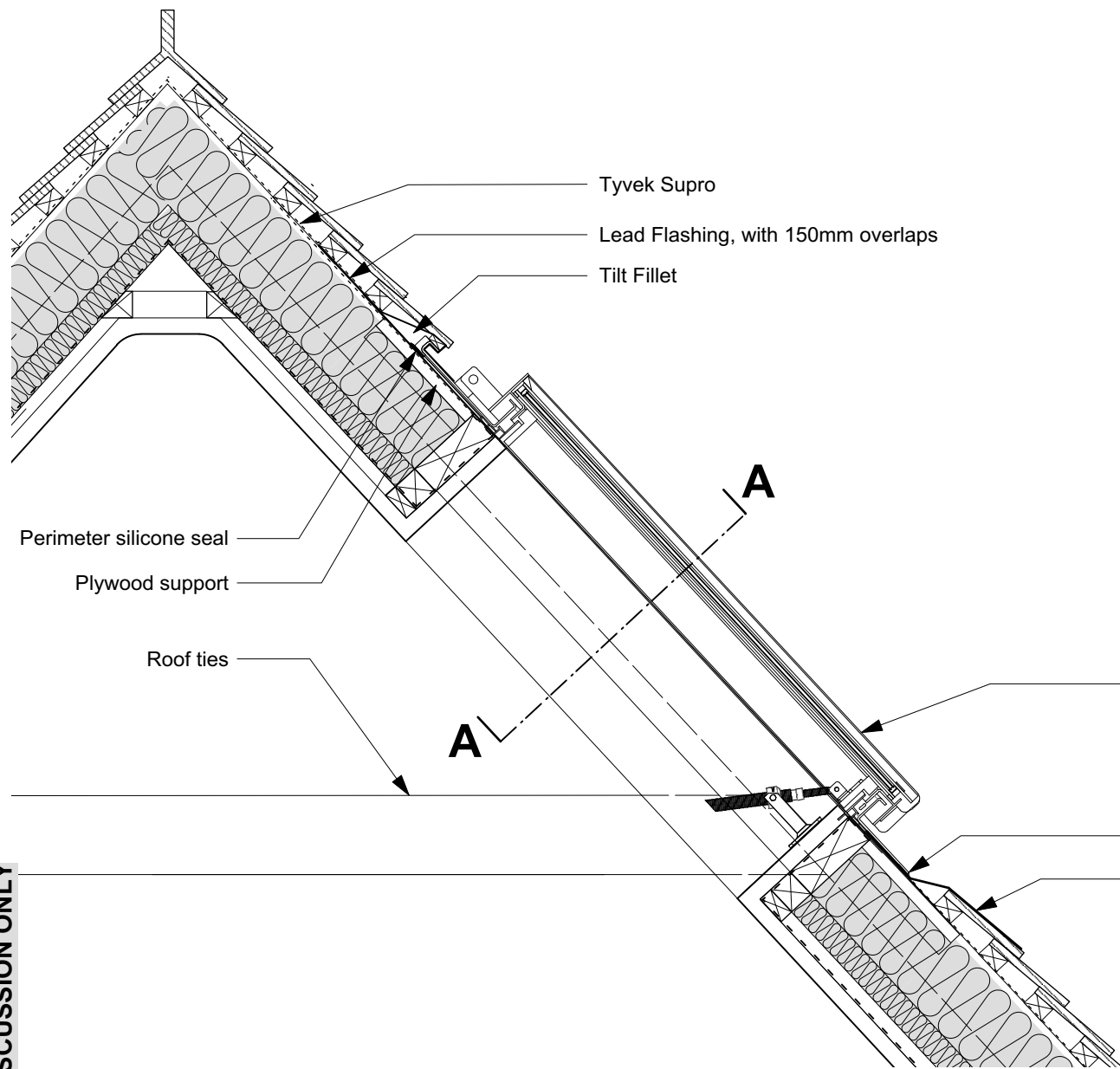
01 603 CONSERVATION ROOF LIGHTS SECTION 1:10
