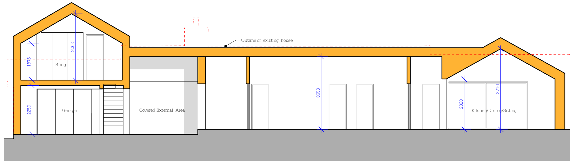
Proposed Section A
