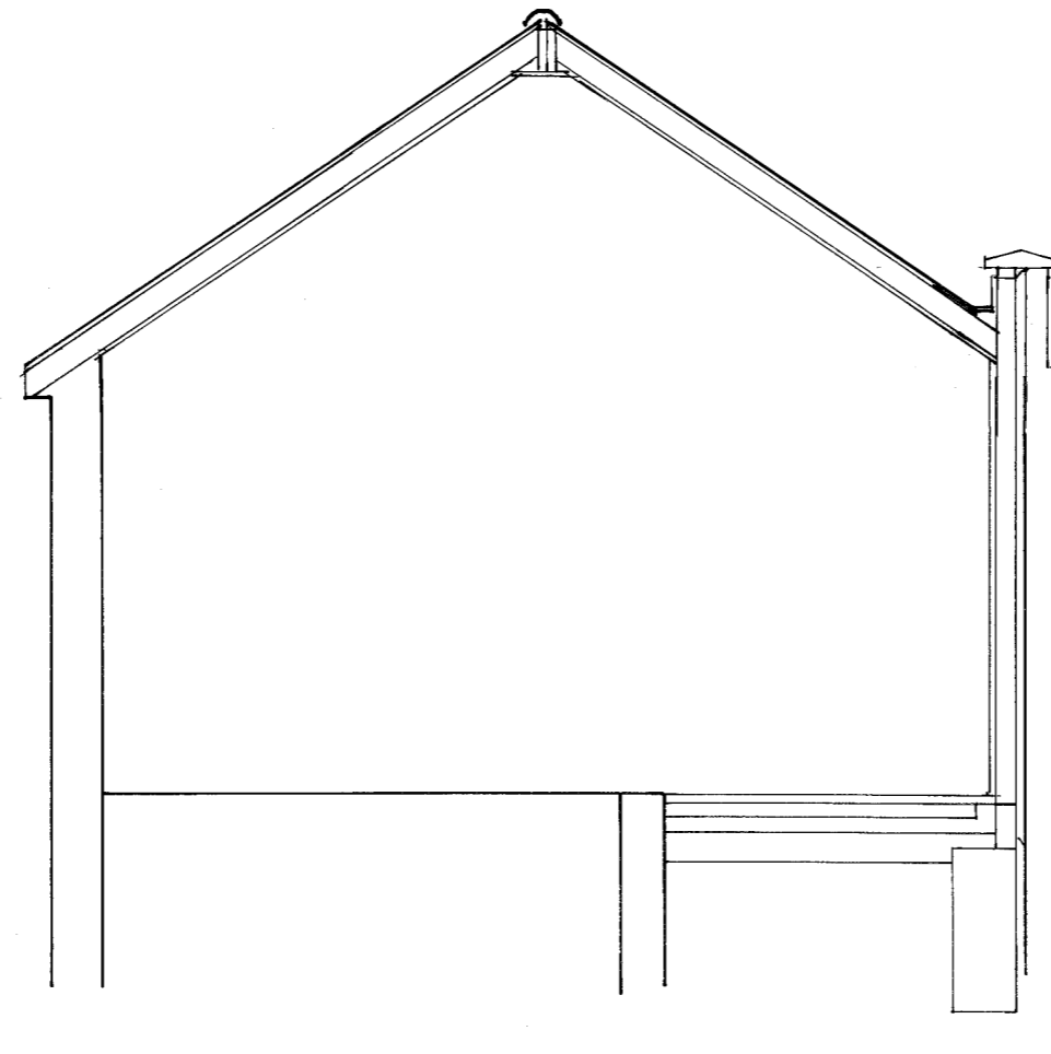
Cross-Section
