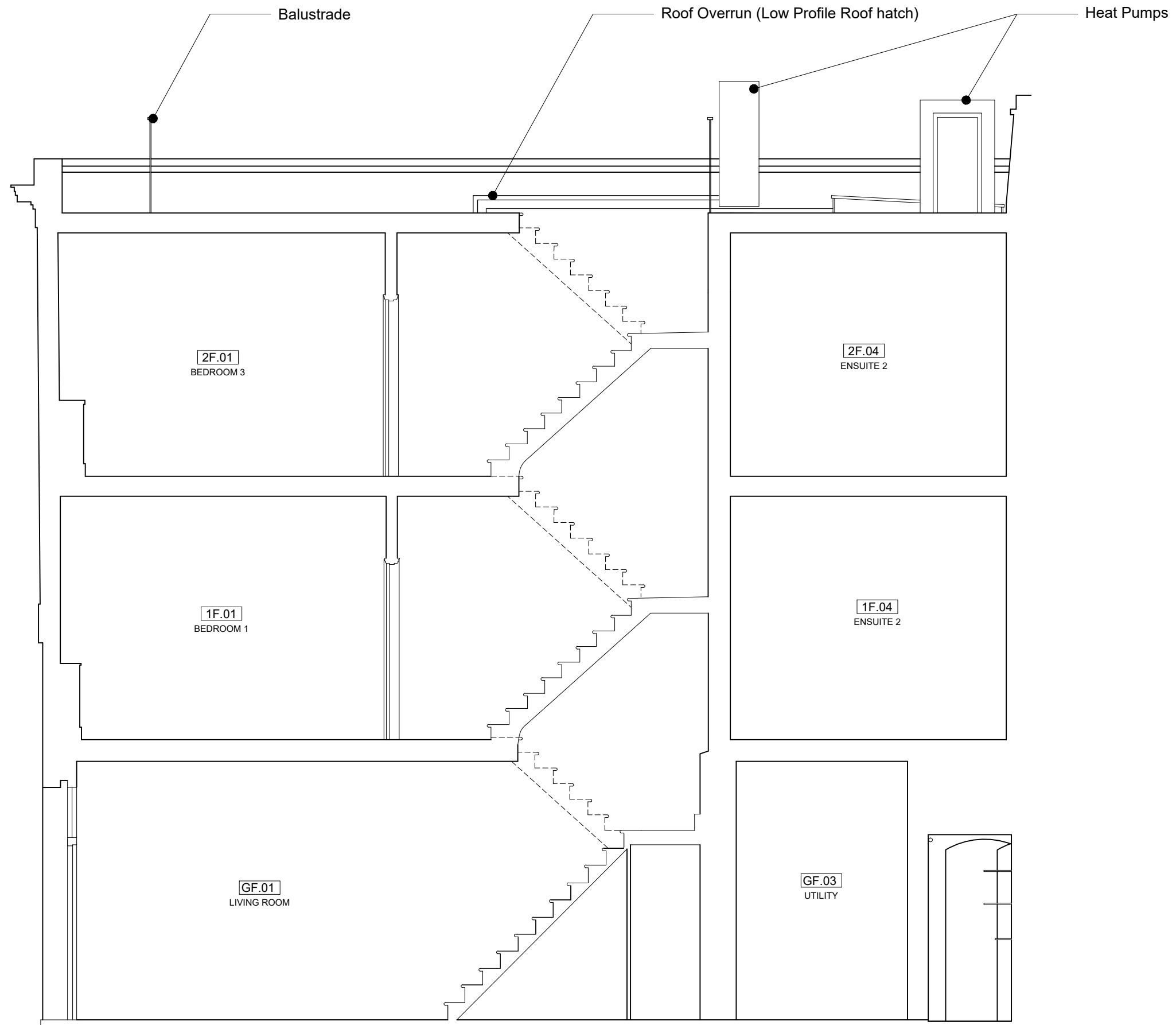
SECTION A-A SECTION
