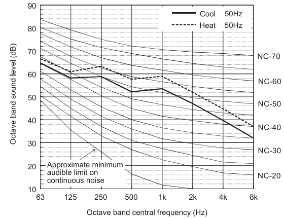
Sound level of PUMY-P300YBM
