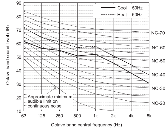
Sound level of PUMY-P250YBM
