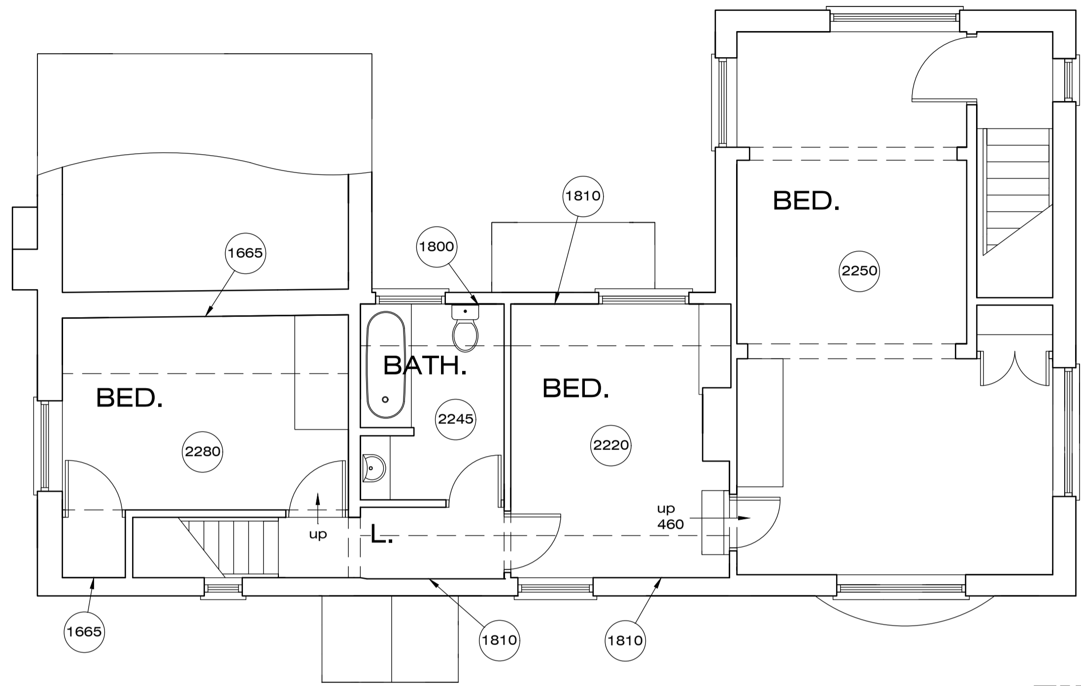
FIRST FLOOR
