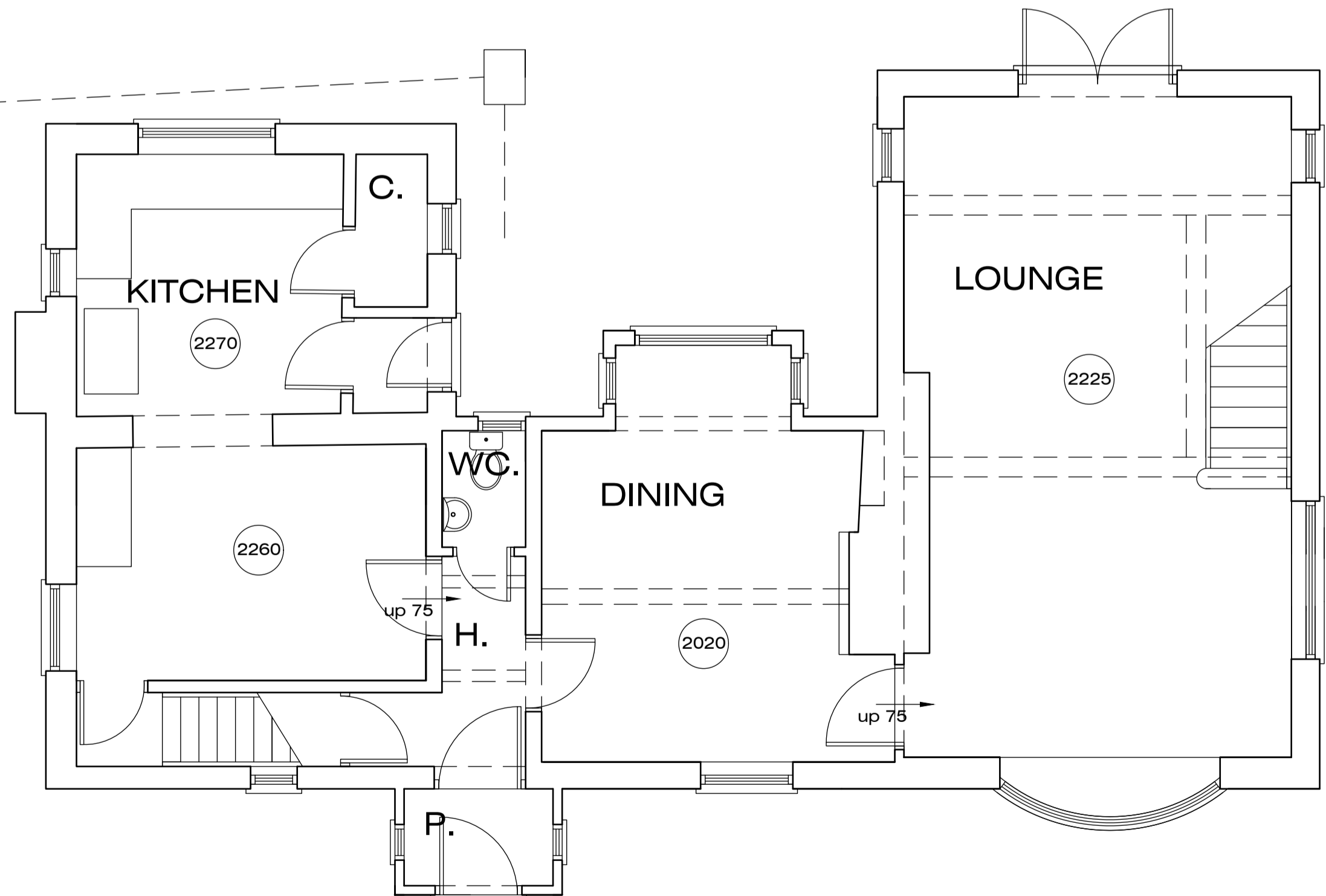
GROUND FLOOR
