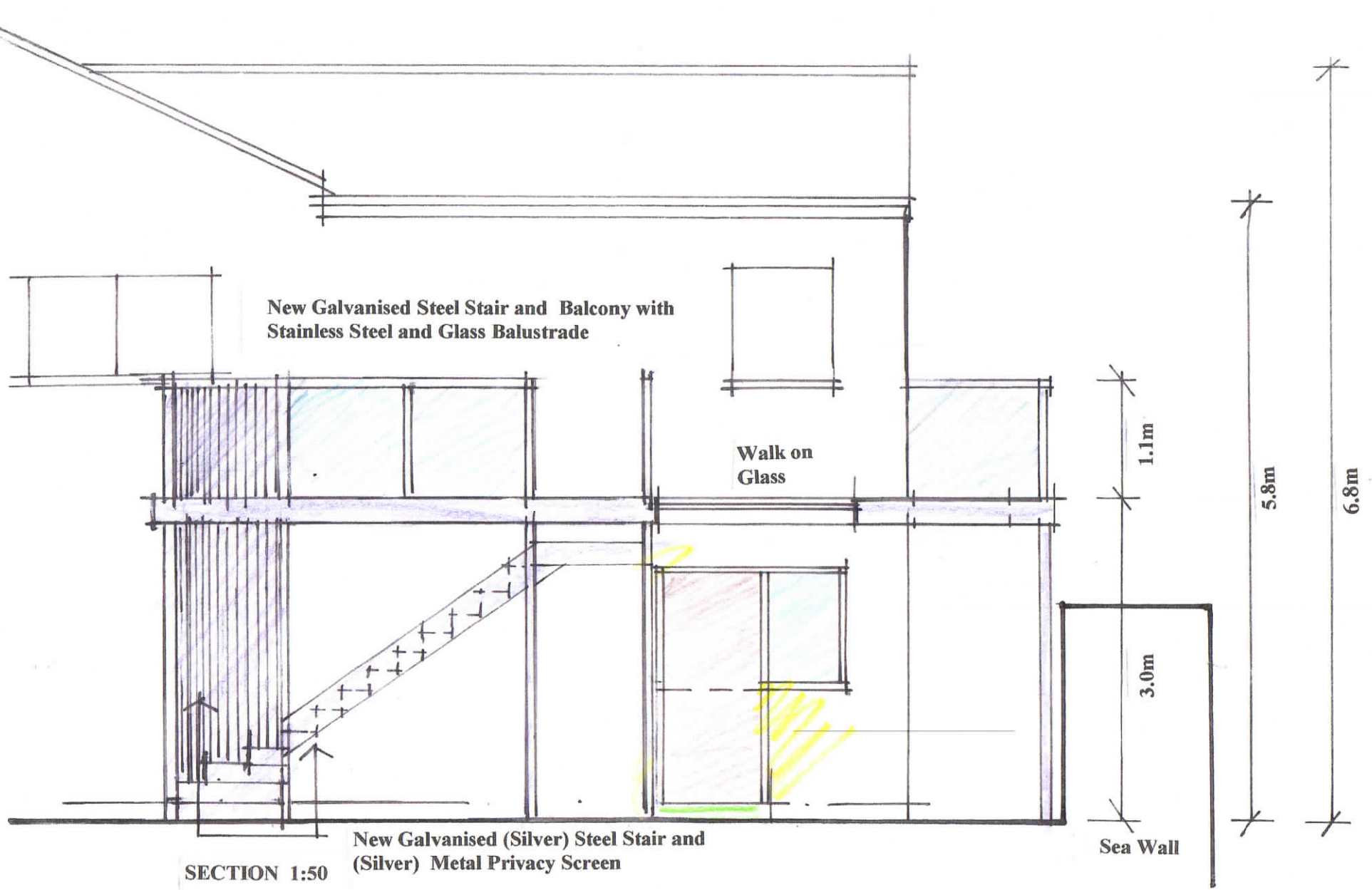
PROPOSED ALTERATIONS AT 4 HARBOUR LANE, GARDENSTOWN. DRWG 06
