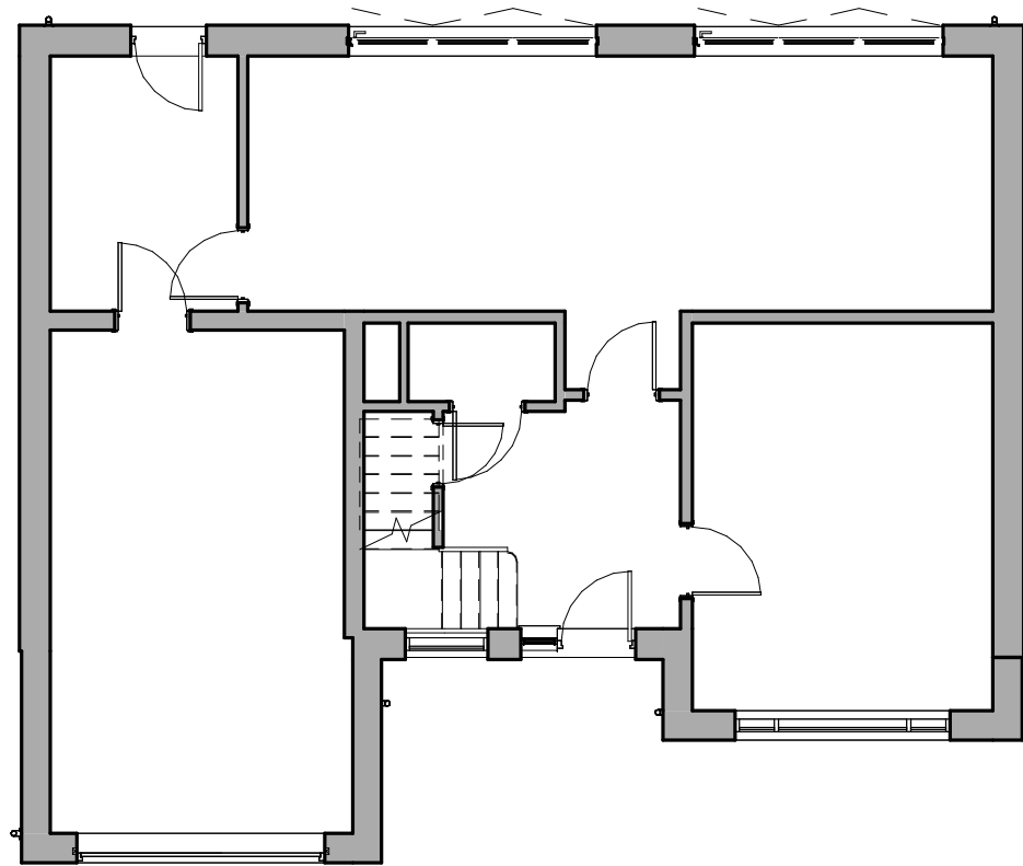
01 GROUND FLOOR - HOUSE TYPE 1 1 : 100
