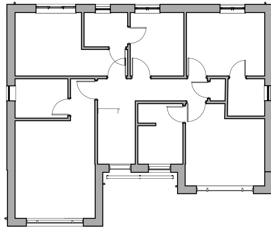
02 FIRST FLOOR - HOUSE TYPE 1 1 : 100
