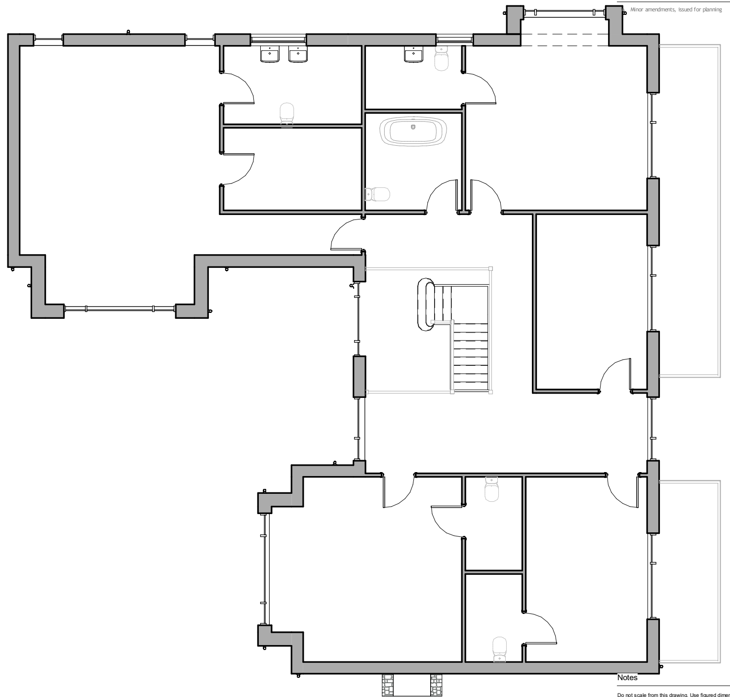
02 FIRST FLOOR - HOUSE TYPE 3 1 : 100
