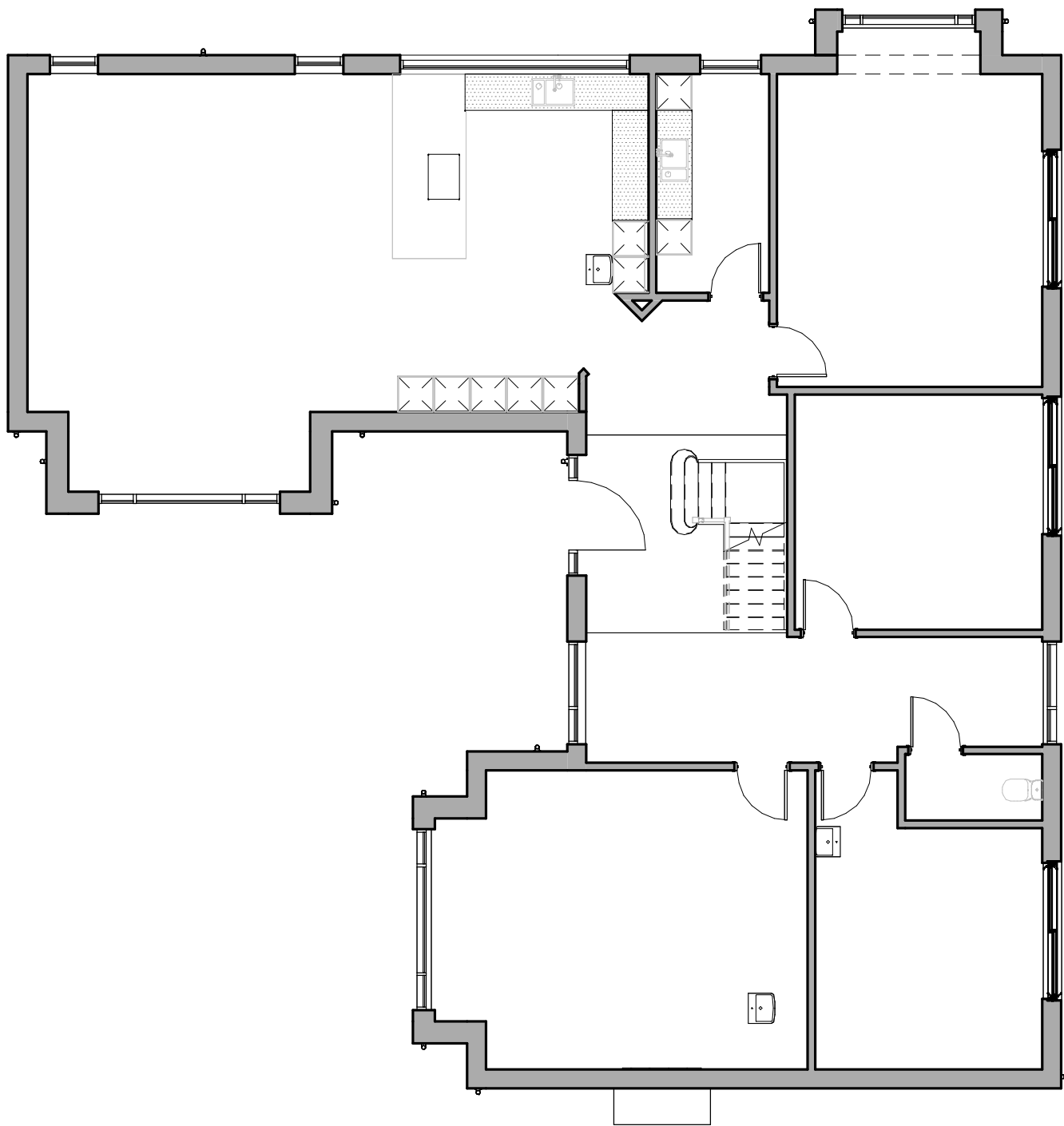
01 GROUND FLOOR - HOUSE TYPE 3 1 : 100
