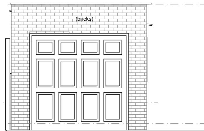
Garage - South Elevation - Existing 1:50
