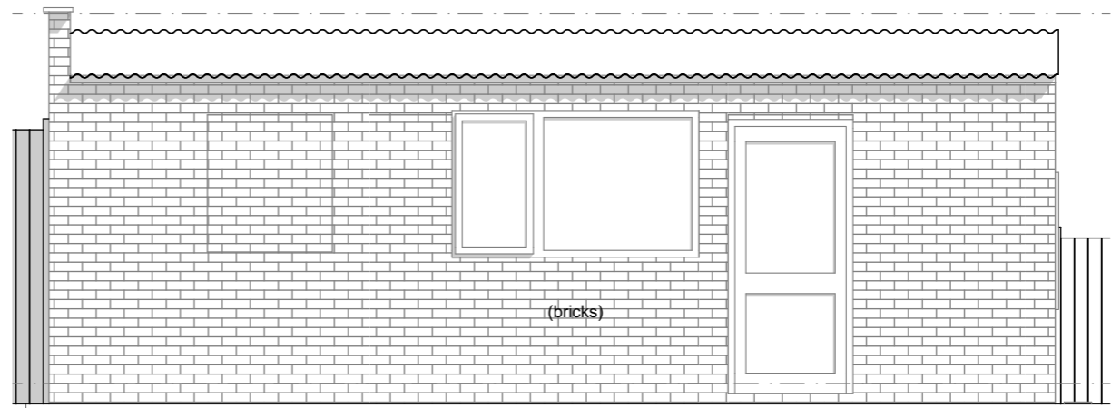
Garage - East Elevation - Existing 1:50
