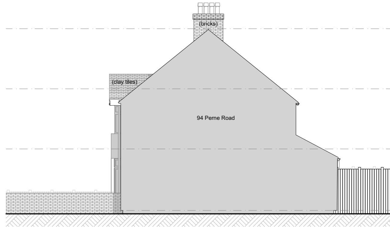
East Elevation - Existing 1:100
