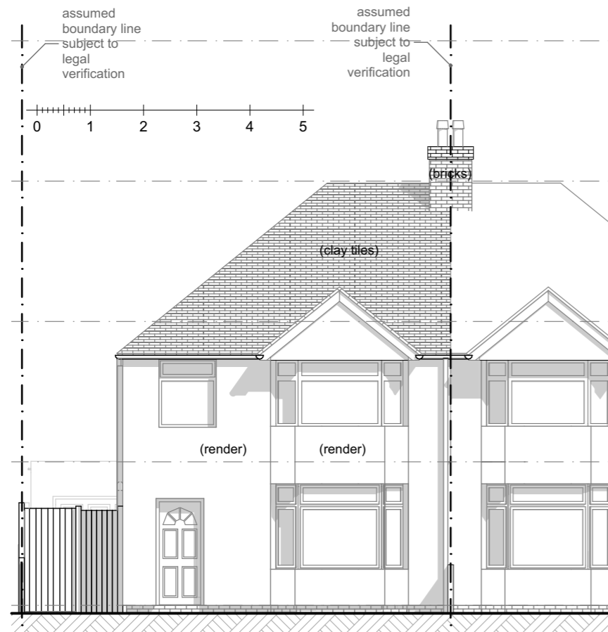
South Elevation - Existing 1:100
