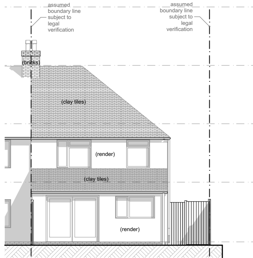
North Elevation - Existing 1:100
