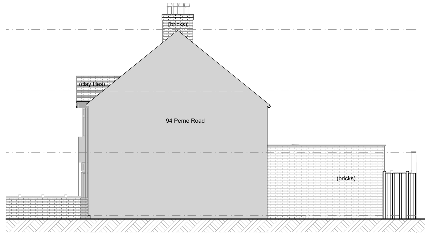
East Elevation - Proposed 1:100
