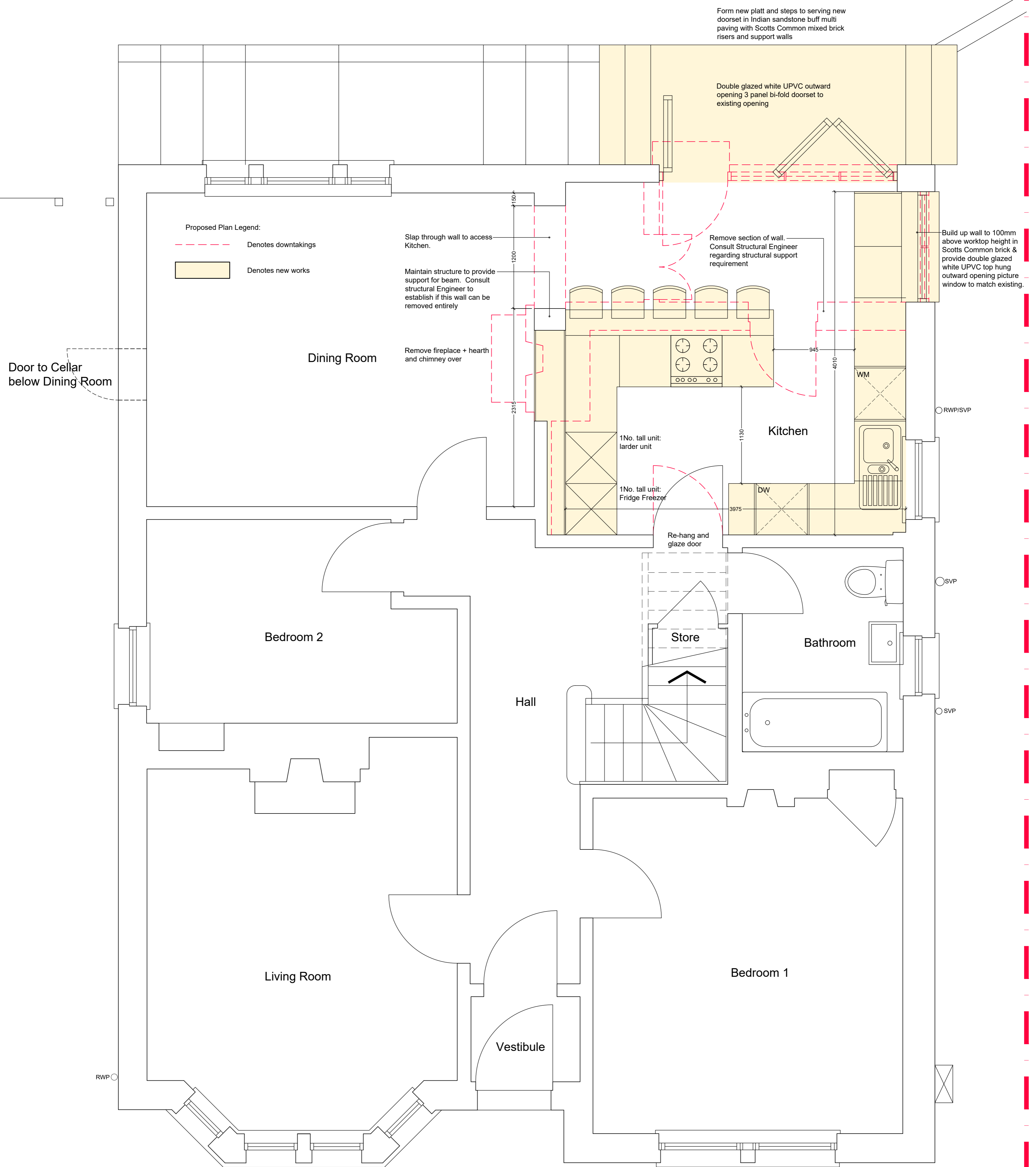
Ground floor plan as proposed 1:25@A1
