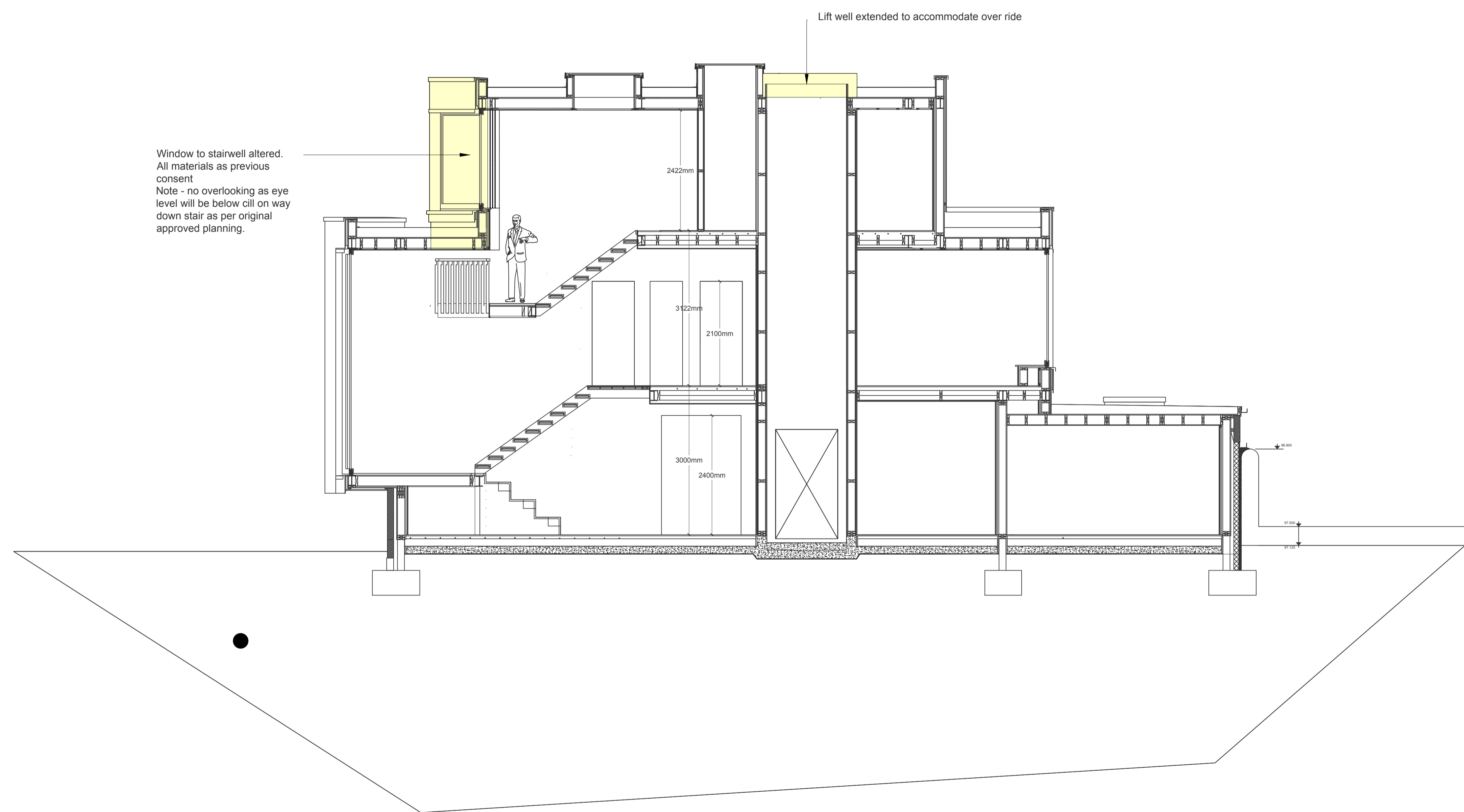
SECTION THRO STAIR
