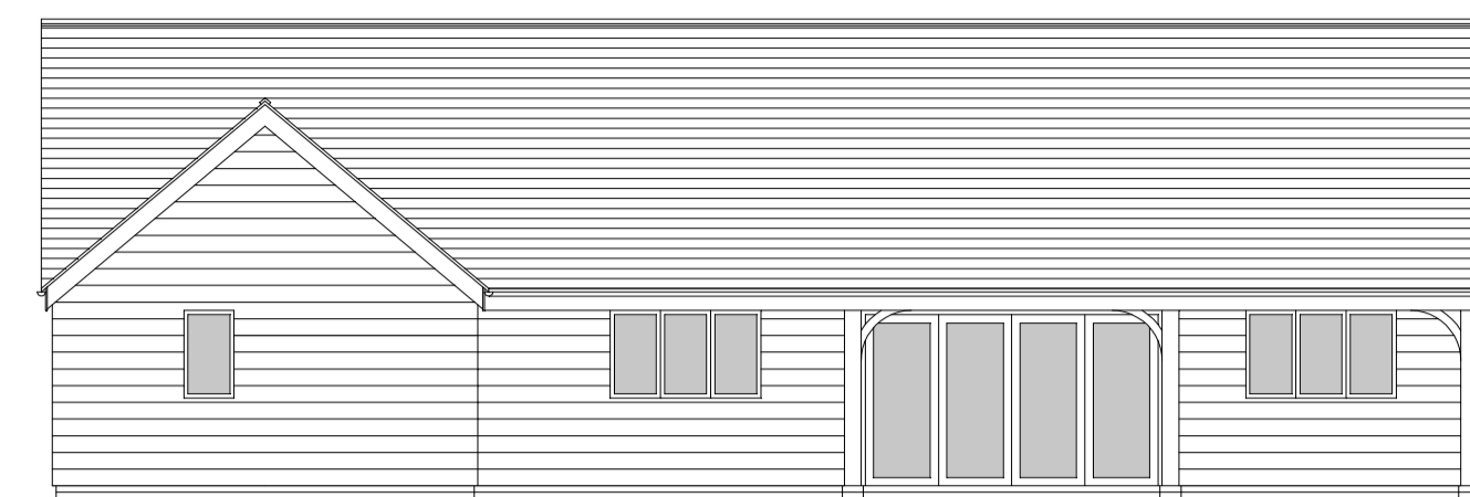
Proposed Rear (North) Elevation 1:100
