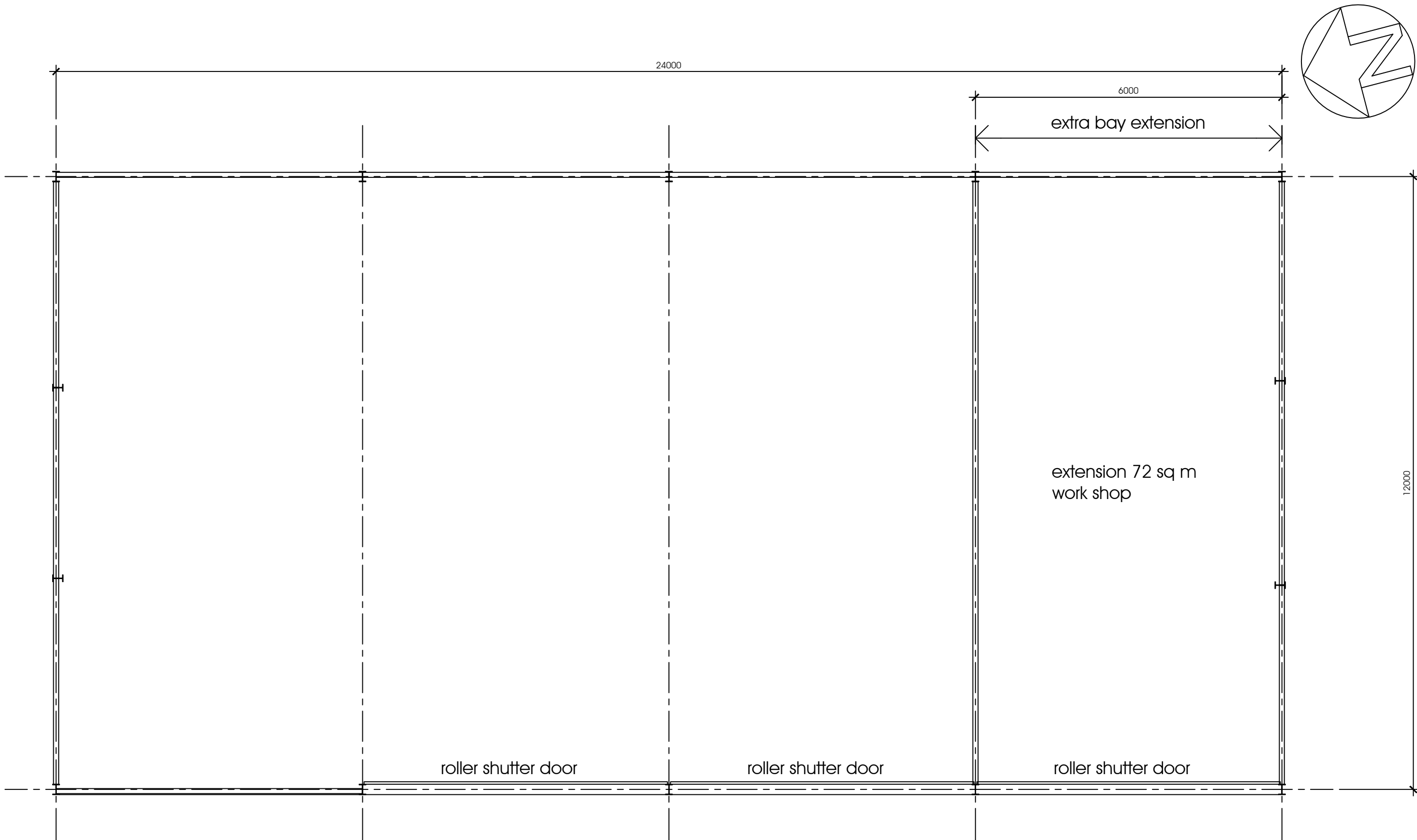
floor plan
