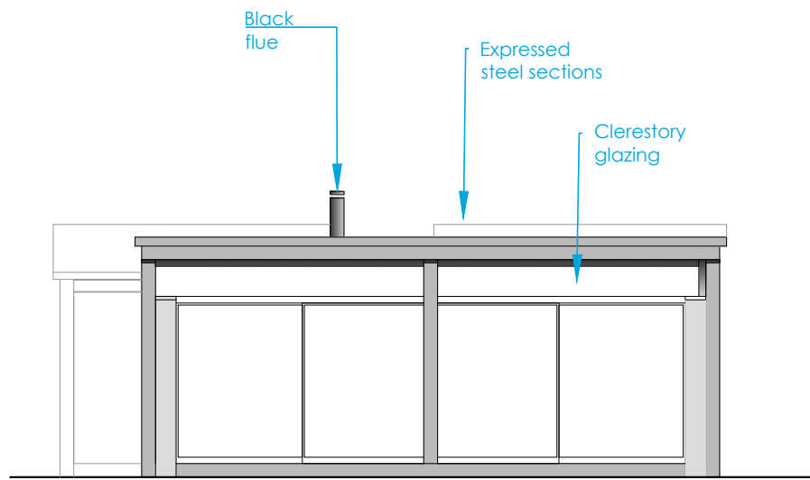
1:100 South West Elevation Unit 1 & 3
