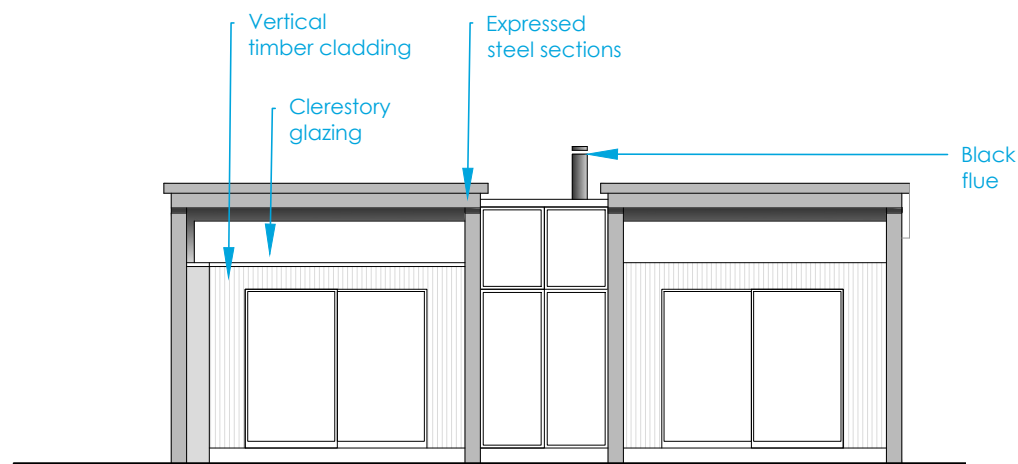
1:100 North East Elevation Unit 1 & 3
