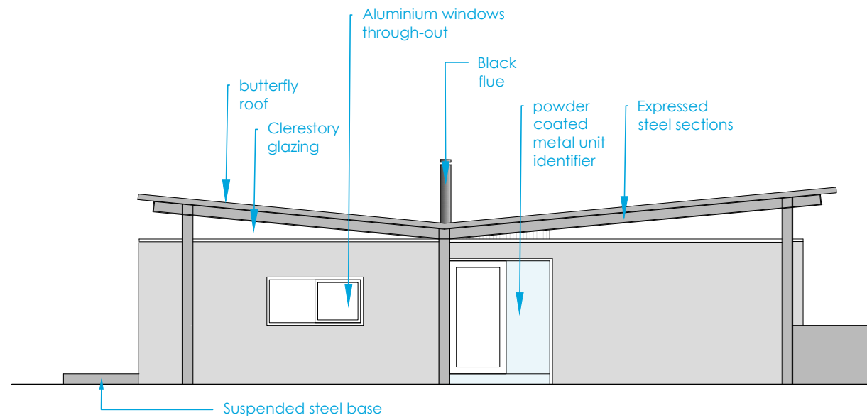
1:100 South East Elevation Unit 1 & 3
