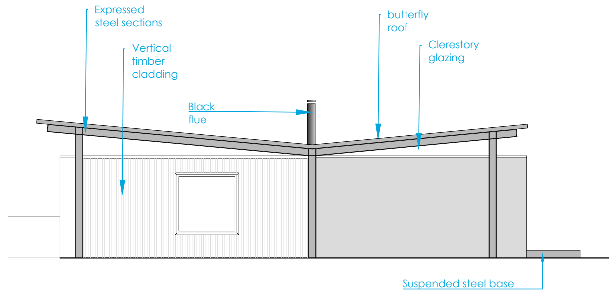
1:100 North West Elevation Unit 1 & 3
