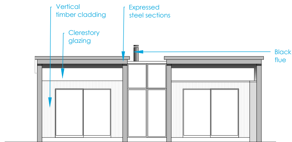
1:100 North East Elevation Unit 2
