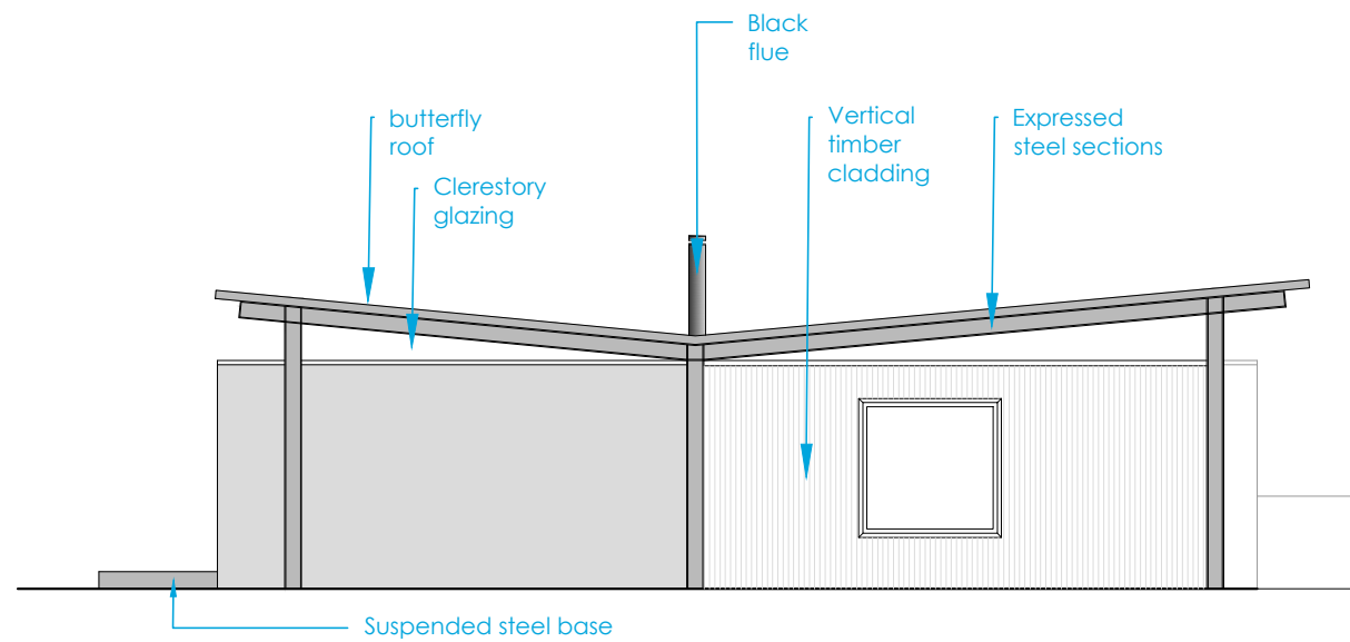
1:100 South East Elevation Unit 2
