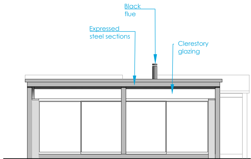
1:100 South West Elevation Unit 2
