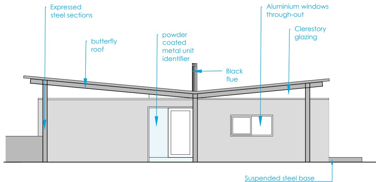
1:100 North West Elevation Unit 2
