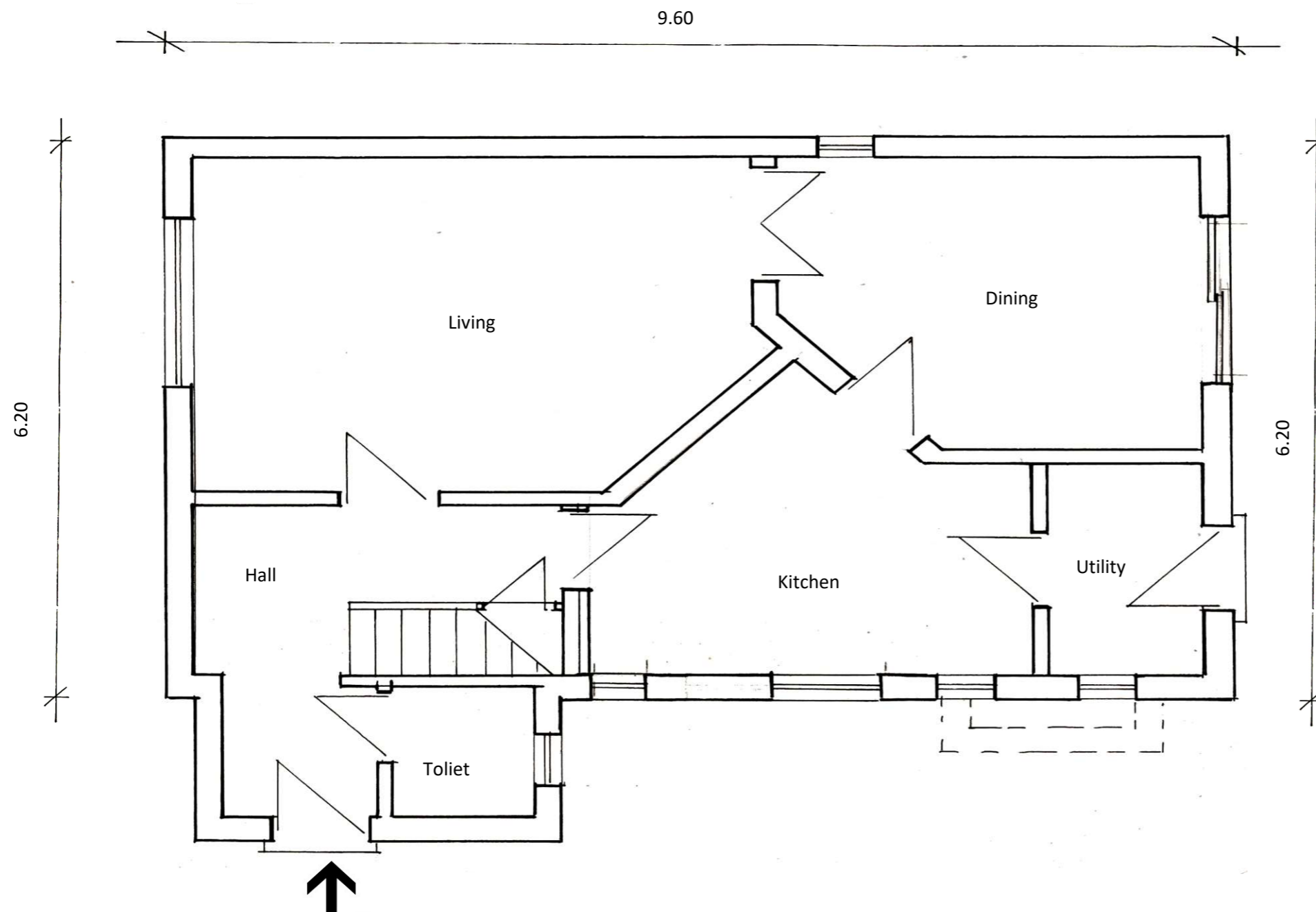
GROUND FLOOR EXISTING
