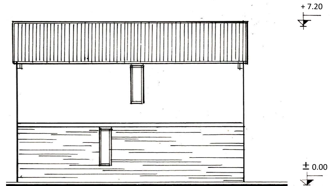
BACK VIEW
