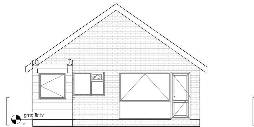
Existing Elevation-Rear
