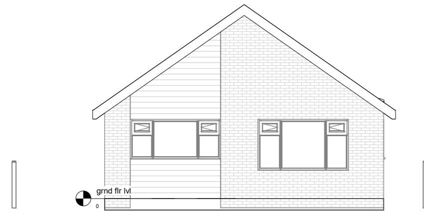
Existing Elevation-Front
