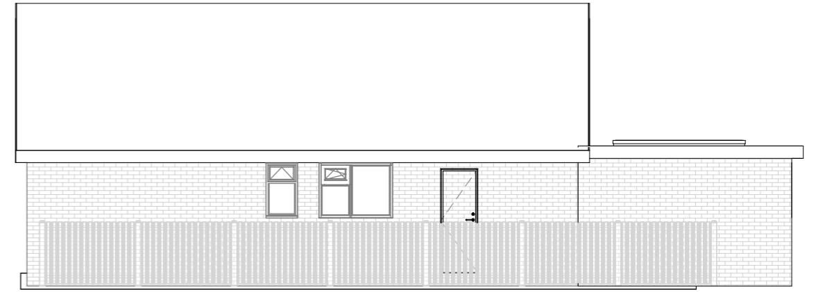
Proposed Elevation-Right side
