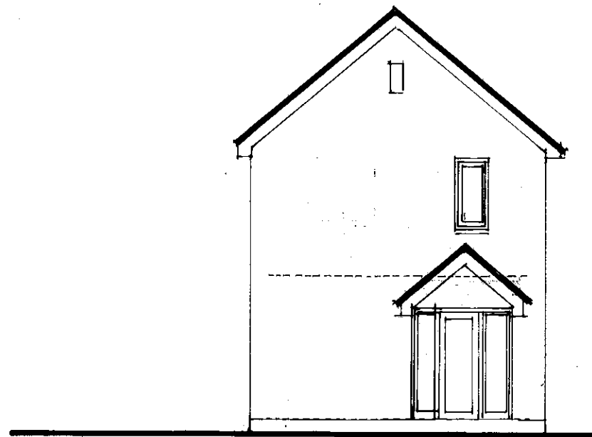
EAST ELEVATION TO LEATHERBOTTLE LANE
