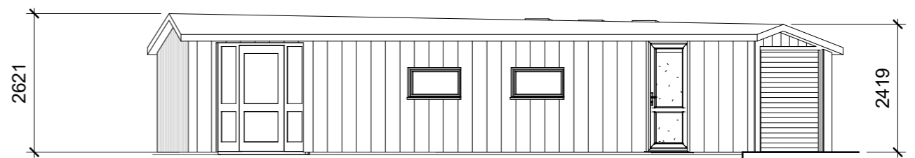
Elevations NORTH
