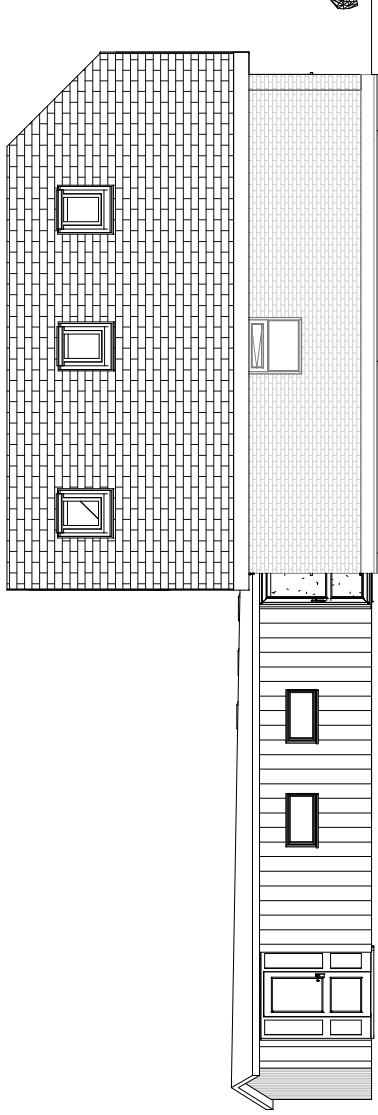
Proposed Elevation NORTH
