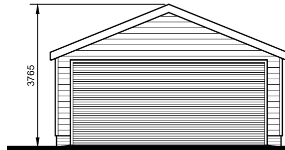
Front Elevation (Southeast)
